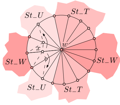
Figure 5: The vertex w is a saddle. The lower star of U sandwiches a component of the lower star of w . By subdividing its edges, we turn w into a regular vertex, replacing it by the new saddle x . The shading shows the lower stars after the subdivision. The arrows indicate the direction in which the values of the new vertices increase.
