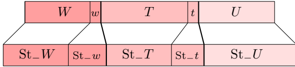
Figure 2: Top: The sequence of vertices is partitioned into W with the last vertex w , T with the last vertex t , and U . Bottom: The sequence of simplices defining the corresponding lower-star filtration.
