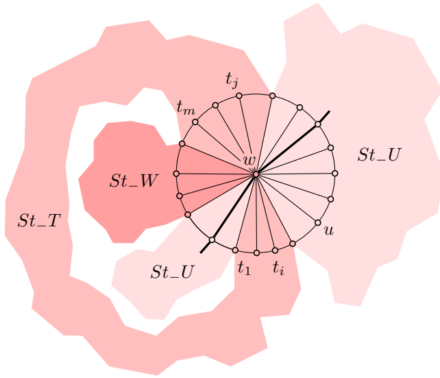
Figure 3: The addition of the lower star of T to the lower star of W creates a non-bounding cycle, which implies that T contains a positive saddle. The partially indicated path passing through w locally separates t_i and t_j .
