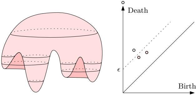
Figure 1: Left: Two embeddings of a 2-manifold \mathbb{M} in \mathbb{R}^3 . The functions f, g : \mathbb{M} \rightarrow \mathbb{R} are the height functions of the light shaded and the combined light and dark shaded embeddings. Right: The dimension 0 persistence diagrams of f and g . The two points below the threshold distance \epsilon from the diagonal are present in the persistence diagram of f but not in that of its \epsilon -simplification g . The other two points appear in both diagrams.
