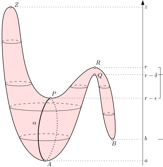
Figure 8: Embedding of the 2-sphere \mathbb{M} in \mathbb{R}^3 such that f : \mathbb{M} \rightarrow \mathbb{R} is its height function. There are two minima, A and B , two saddles, P and Q , and two maxima, R and Z . The two ascending paths from A to P decompose \mathbb{M} into a left and a right hemisphere.
