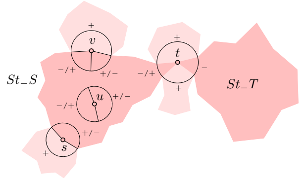
Figure 7: Reordering the vertices in T . Before the reordering, all vertices in T are regular except for s and t . After reordering, all vertices in T are regular. Plus and minus signs distinguish between upper and lower links. The cases in which the reordering swaps upper and lower links are marked by two signs.
