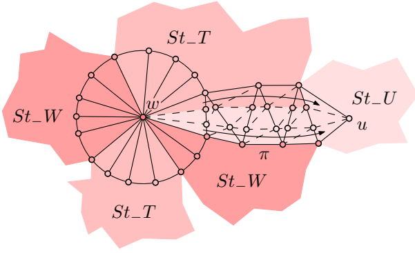
Figure 6: Connecting w to U in case the upper link of w has only vertices in T . The subdivision creates two monotonically increasing paths of new vertices parallel to the path \pi in the link of T . The shading shows the lower stars after the subdivision.
