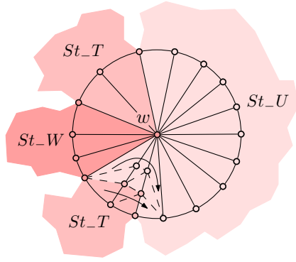
Figure 4: The vertex w is regular. Before the subdivision, St_{-T} \cap Lk w is not contractible while (St_{-T} \cap Lk w) \cup Lk_{-w} is. By subdividing, we reduce the problem to the case in which St_{-T} \cap Lk w is contractible. The new edges are dashed and the lower stars after subdivision are indicated by the shading. The arrows indicate the direction in which the values of the new vertices increase.
