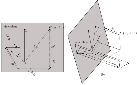
Figure 1: Parallel projection definition from 3D to 2D. (a) Relationship between 3D and 2D coordinates of a point. (b) Parallel projection of the 3D reference system onto the 2D view plane.
