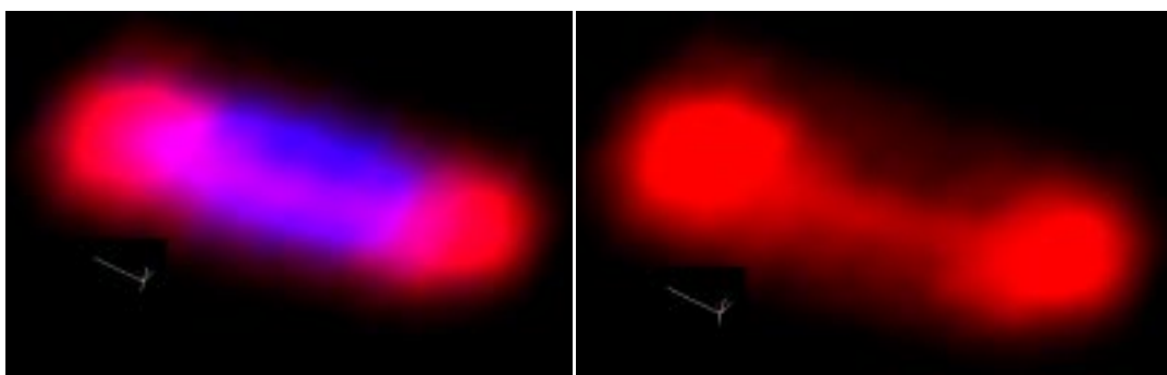
Figure 2: 5D interaction energy scalar field (Red=attraction, Blue=repulsion, Green=free movement). Same view as is figure 1 but highlighting only some of the energy components.
