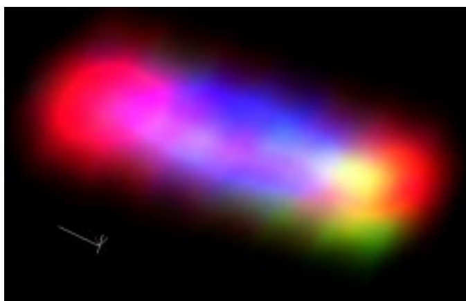
Figure 1: 5D interaction energy scalar field (Red=attraction, Blue=repulsion, Green=free movement). The axes configuration is reported on the bottom left (the stretched axis corresponds to a rotational degree of freedom).
