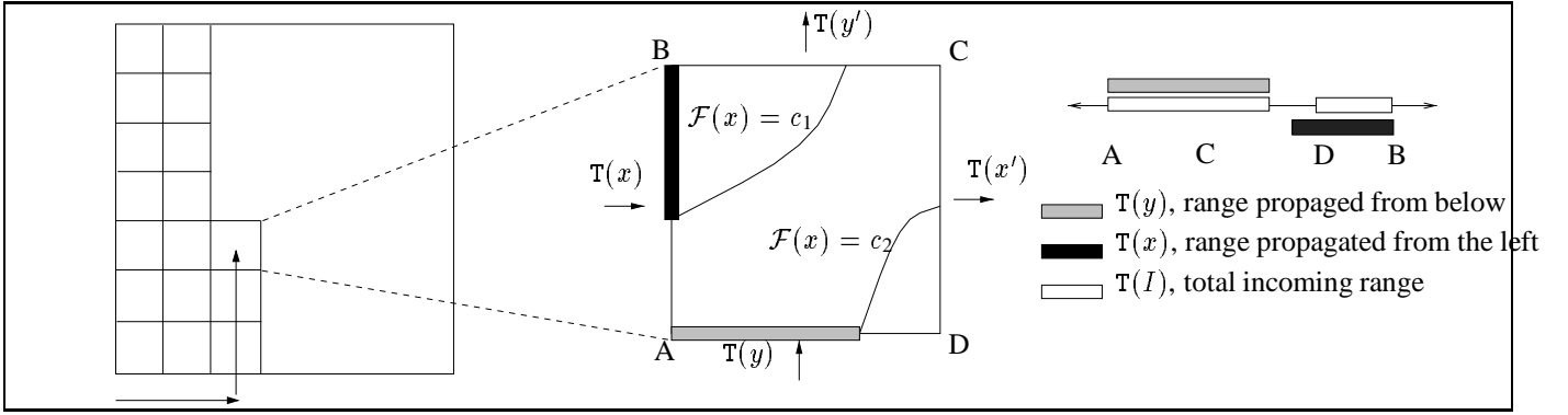
FIGURE 3: Illustration of range propagation for a single cell
